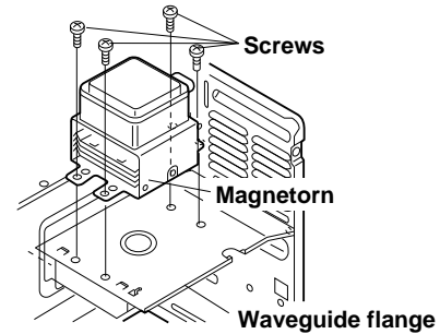
Figure C-1. Magnetron replacement
