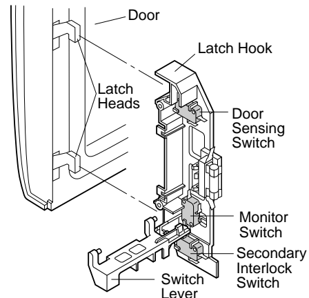
Figure C-6. Latch Switch Adjustments
