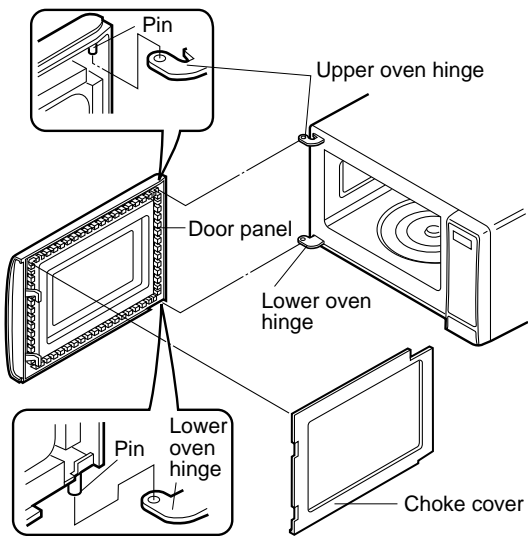
Figure C-8. Door Replacement
