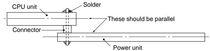
Figure C-4. Side view of CPU unit and Power unit
