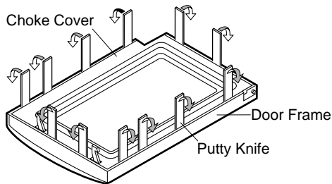
Figure C-7. Door Disassembly
