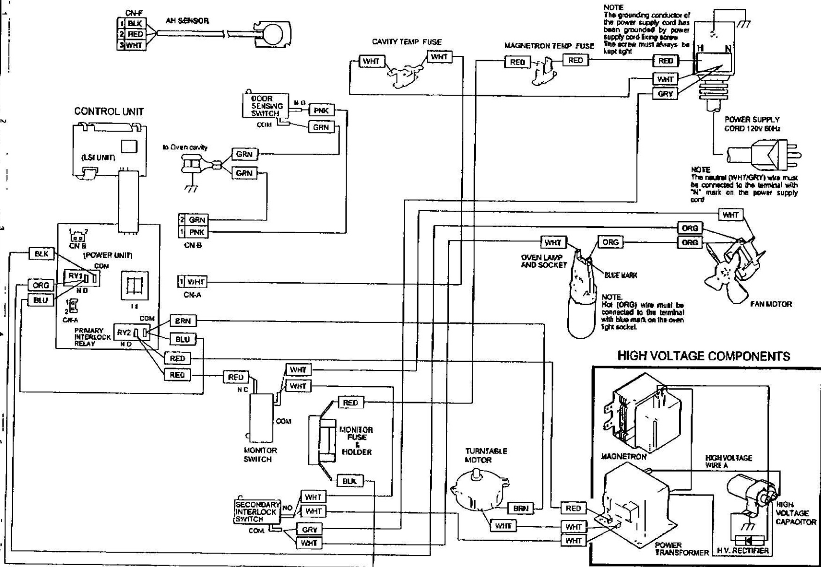
Figure S-1. Pictorial Diagram R-430DK/DW/DQ
